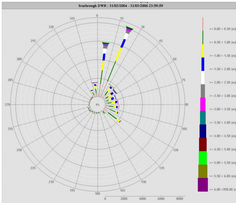
Figure 2.14 Wave Rose at Scarborough DWR site
