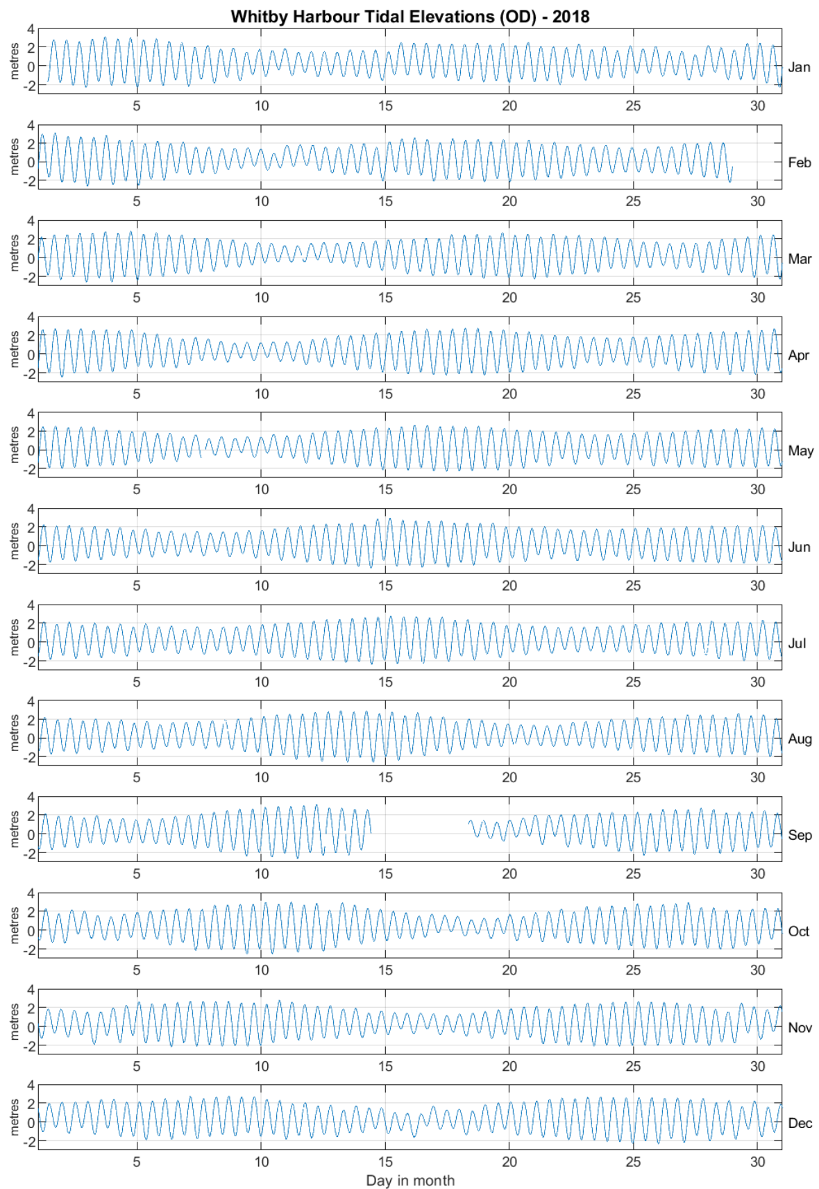
Figure 2: Whitby Harbour tidal elevations for 2018 relative to Ordnance Datum
