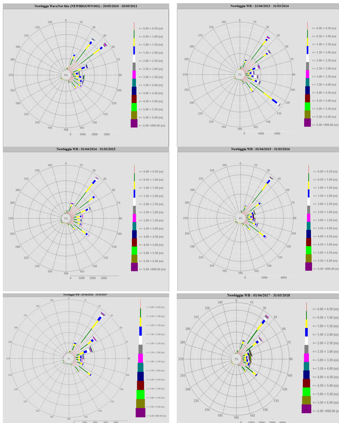
Figure 2.2 Wave roses for Newbiggin WB original deployment in 2010/11 and new data for 2013/14, 2014/15, 2015/16, 2016/17, 2017/18 and 2018/19.
