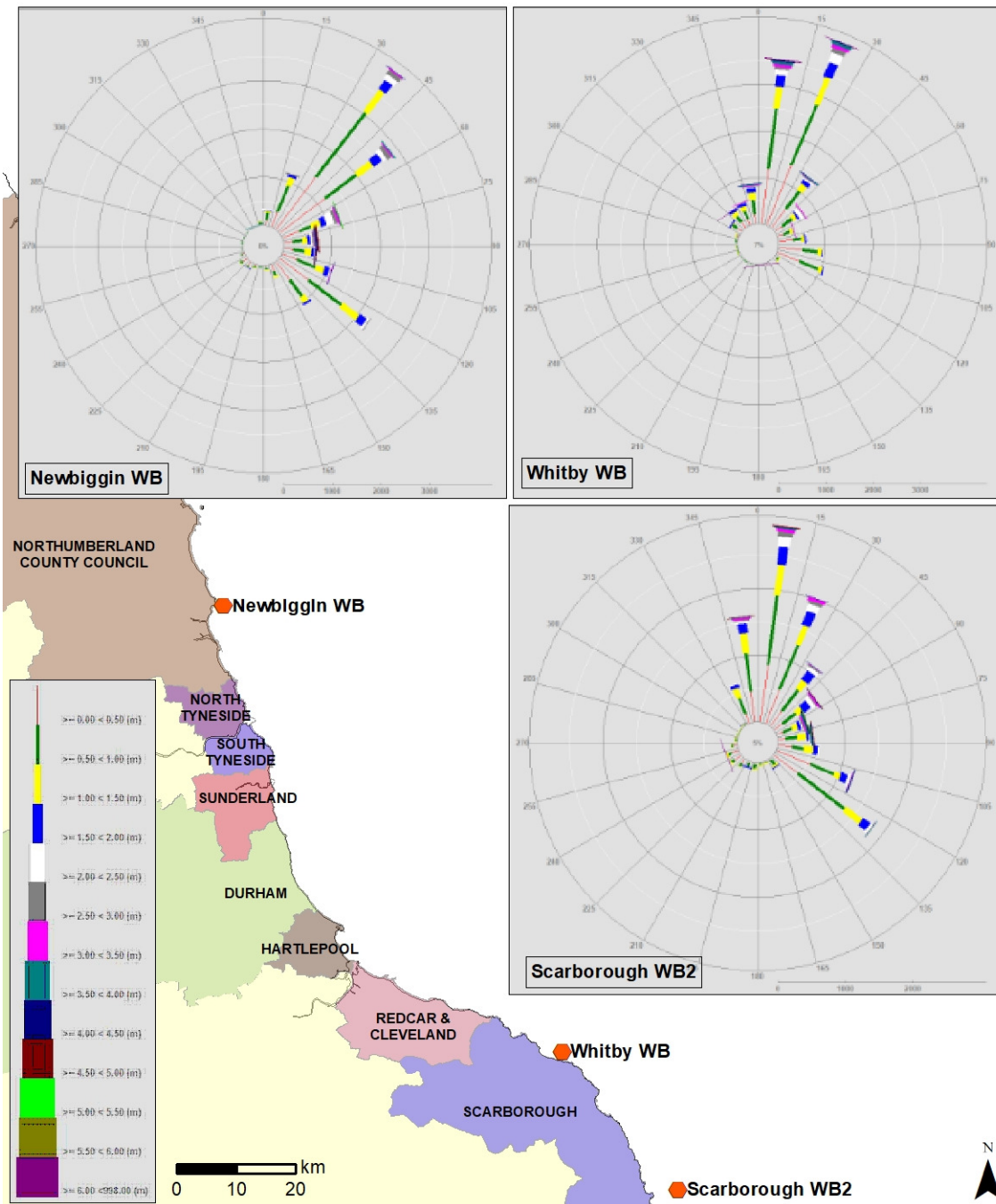
Figure 4.1 Wave Roses (2018/19) from Newbiggin Ness, Whitby and Scarborough
