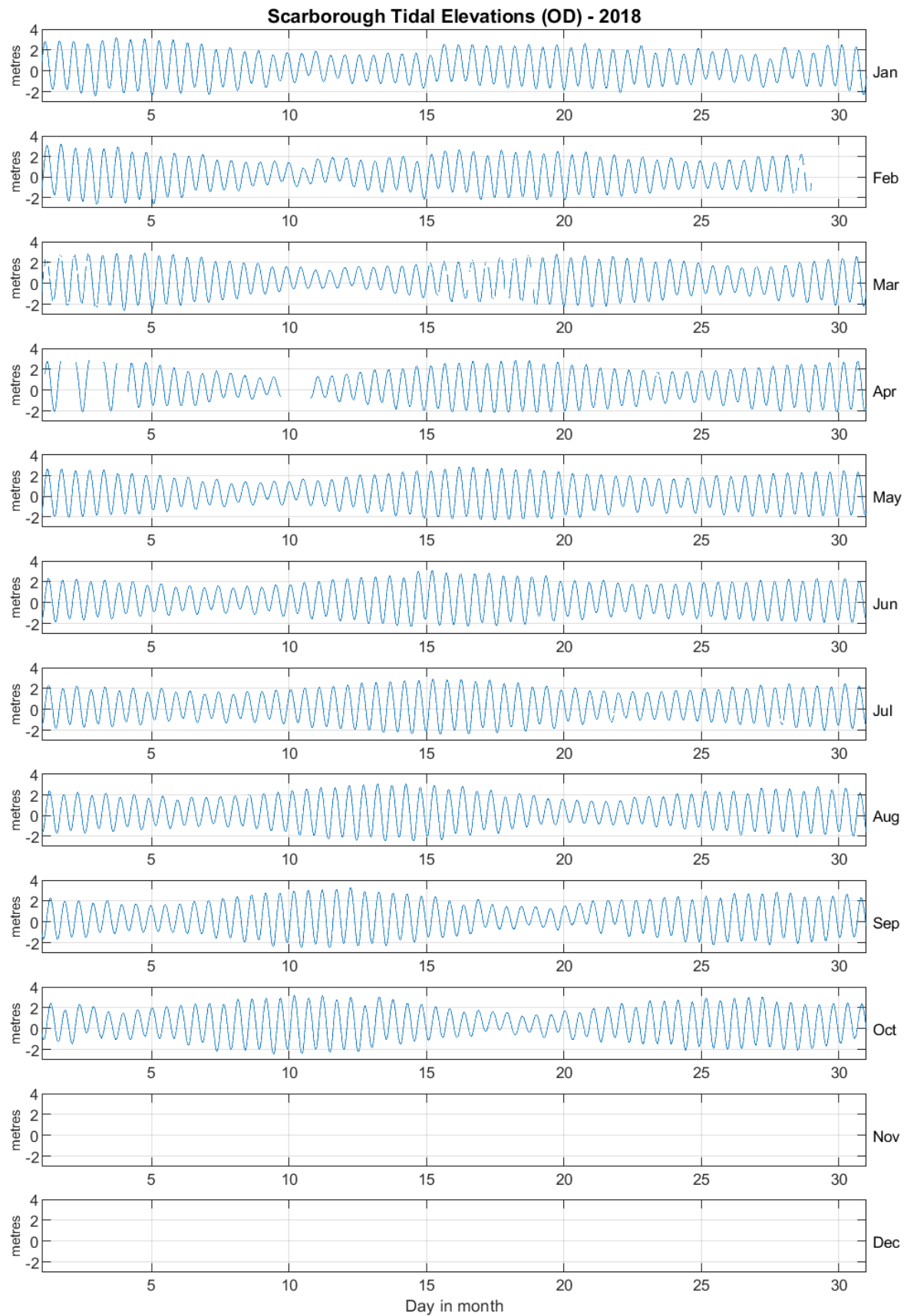
Figure 2: Scarborough tidal elevations for 2018 relative to Ordnance Datum
