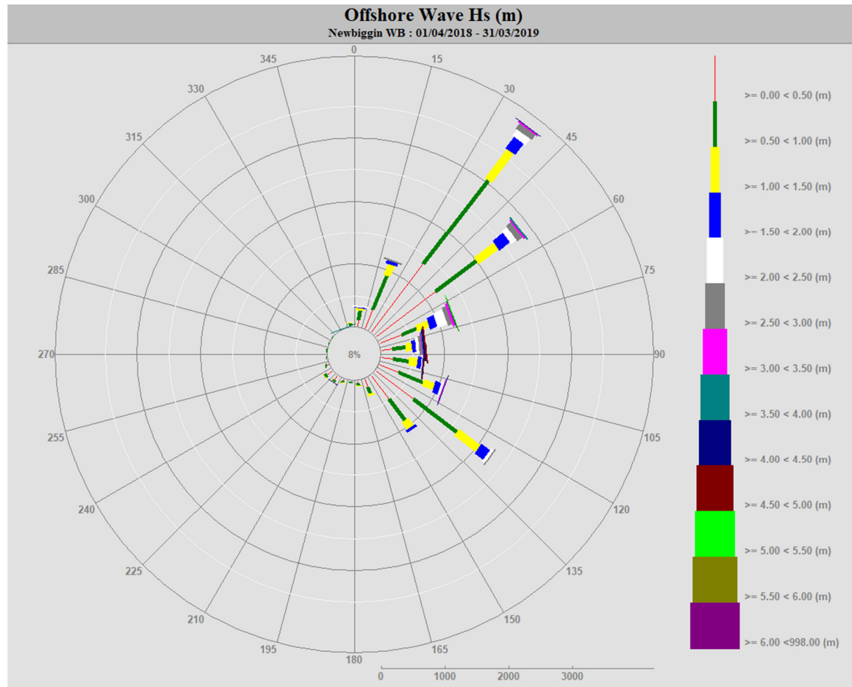
Wave Rose for Newbiggin Wave Buoy 2018-19
