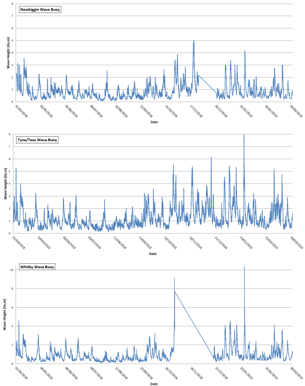
Figure 4.2 Wave height data for 2018-19 in Cell 1
