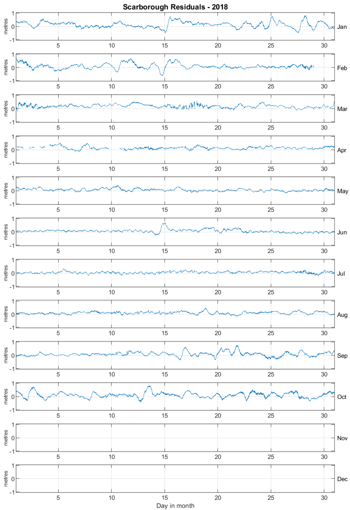
Figure 1: Scarborough residuals for 2018
