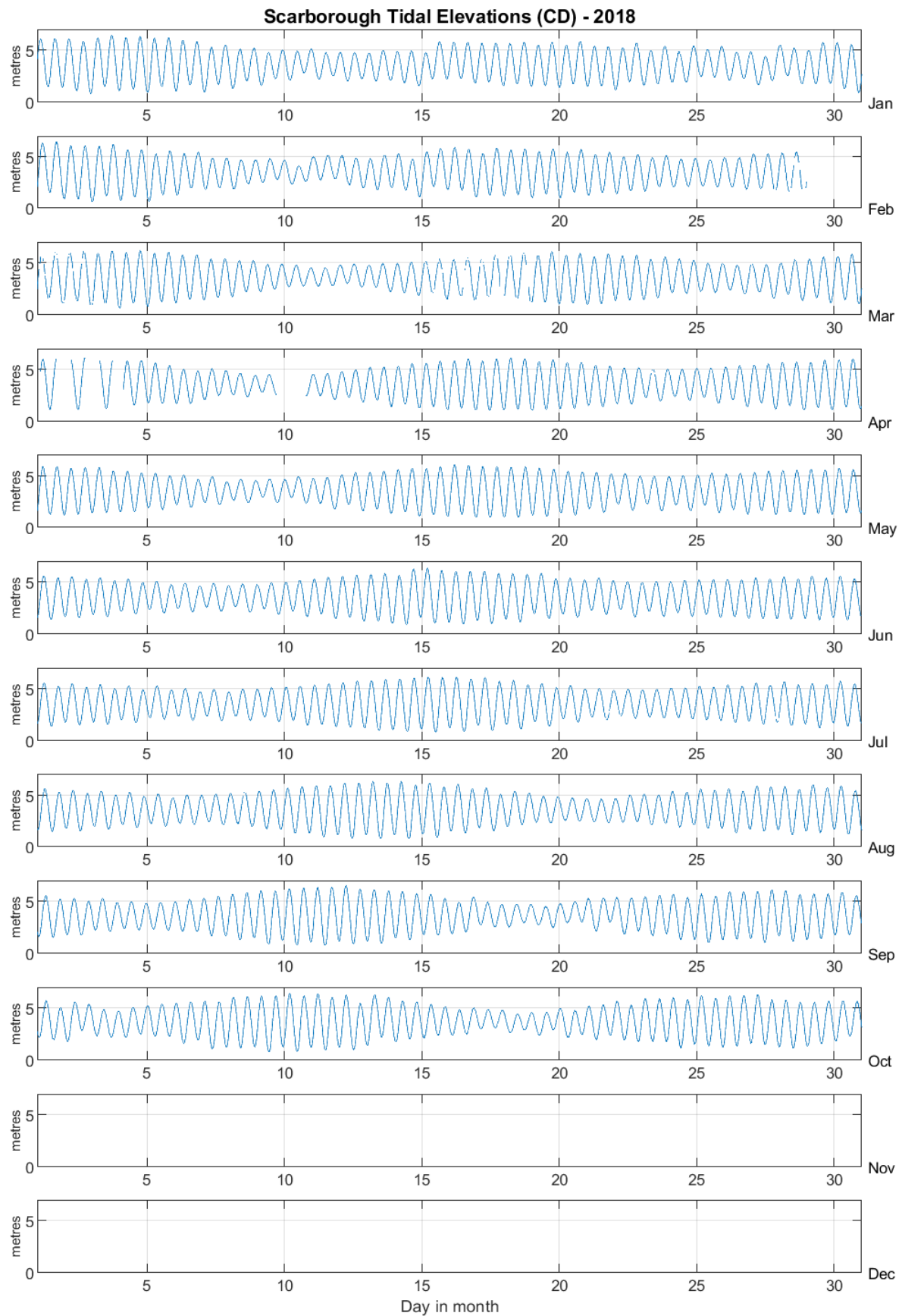
Figure 3: Scarborough tidal elevations for 2018 relative to Chart Datum
