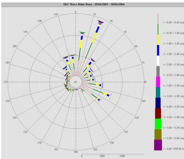
Figure 2.15 Wave Rose at Scarborough SBC site
