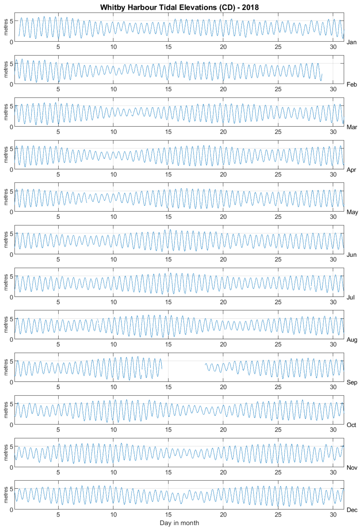
Figure 3: Whitby Harbour tidal elevations for 2018 relative to Chart Datum
