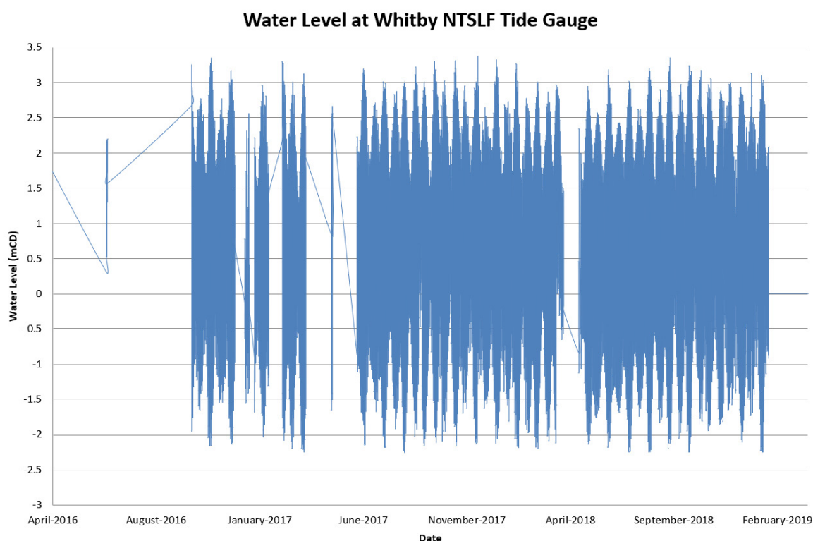
Figure 2.11 Water Level data availability at Whitby NTSLF tide gauge site for 2016-2019
