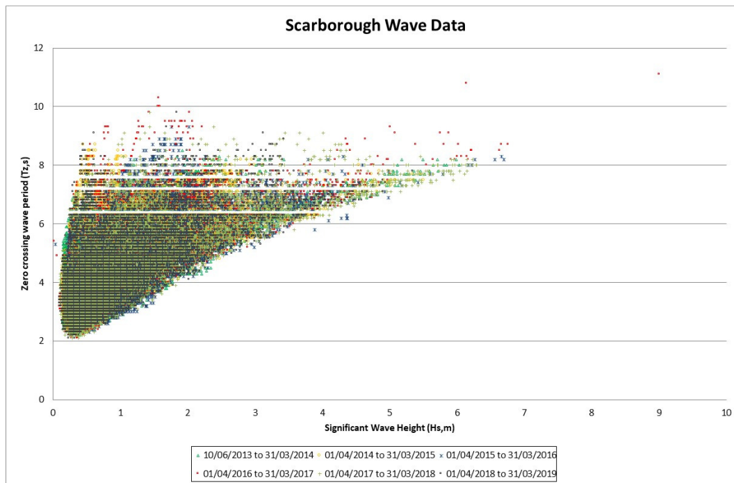
Figure 2.13 Scatter plot of Wave Height Vs Peak Period offshore Scarborough
