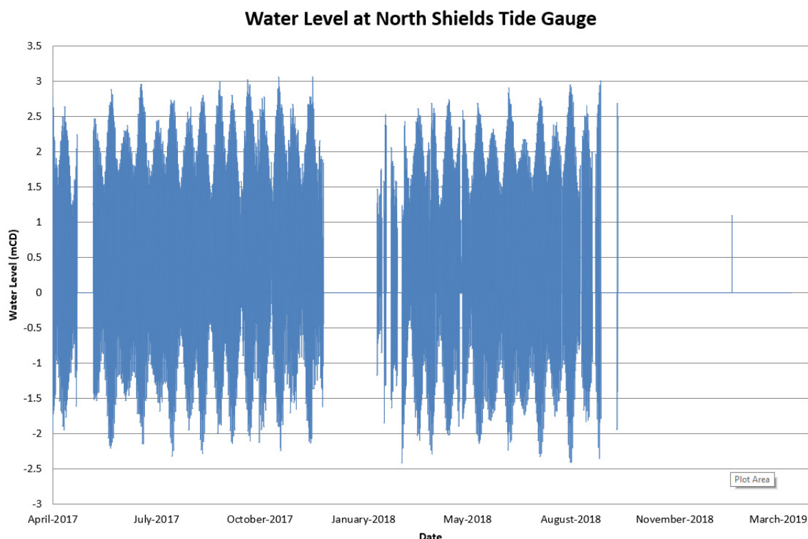
Figure 2.3 Plot of water level data availability for 2017-19 at North Shields NTSLF Tide Gauge
