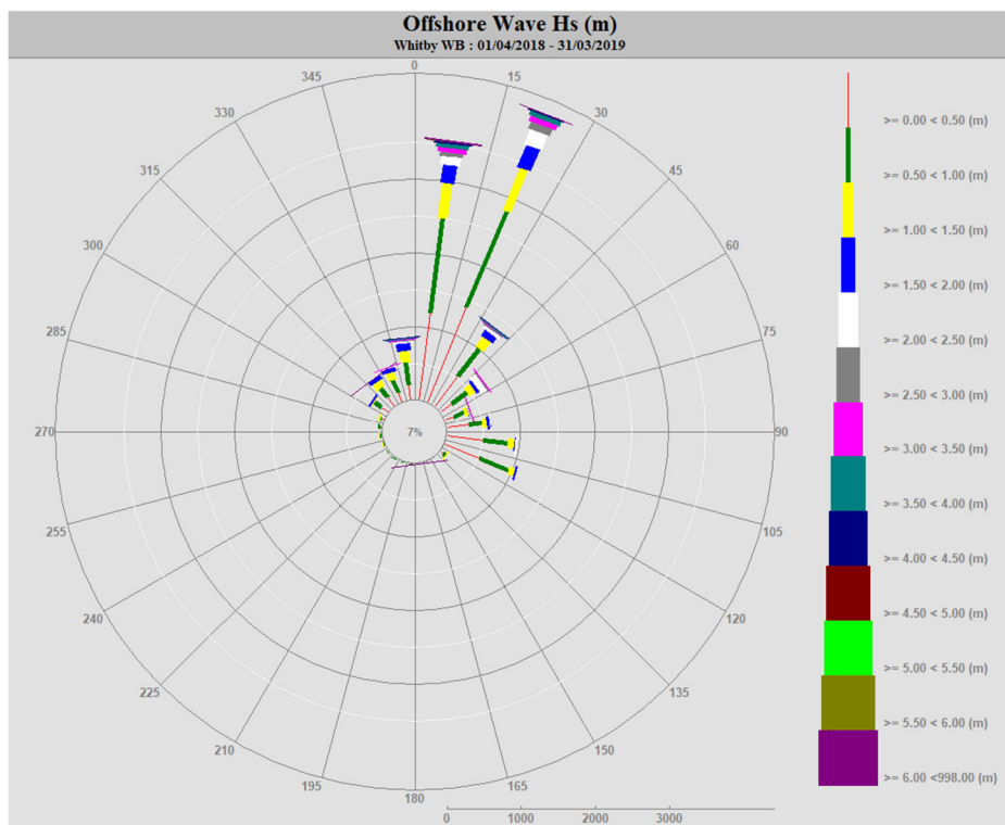
Figure 2.9 (continued) Wave Roses at Whitby wave buoy site
