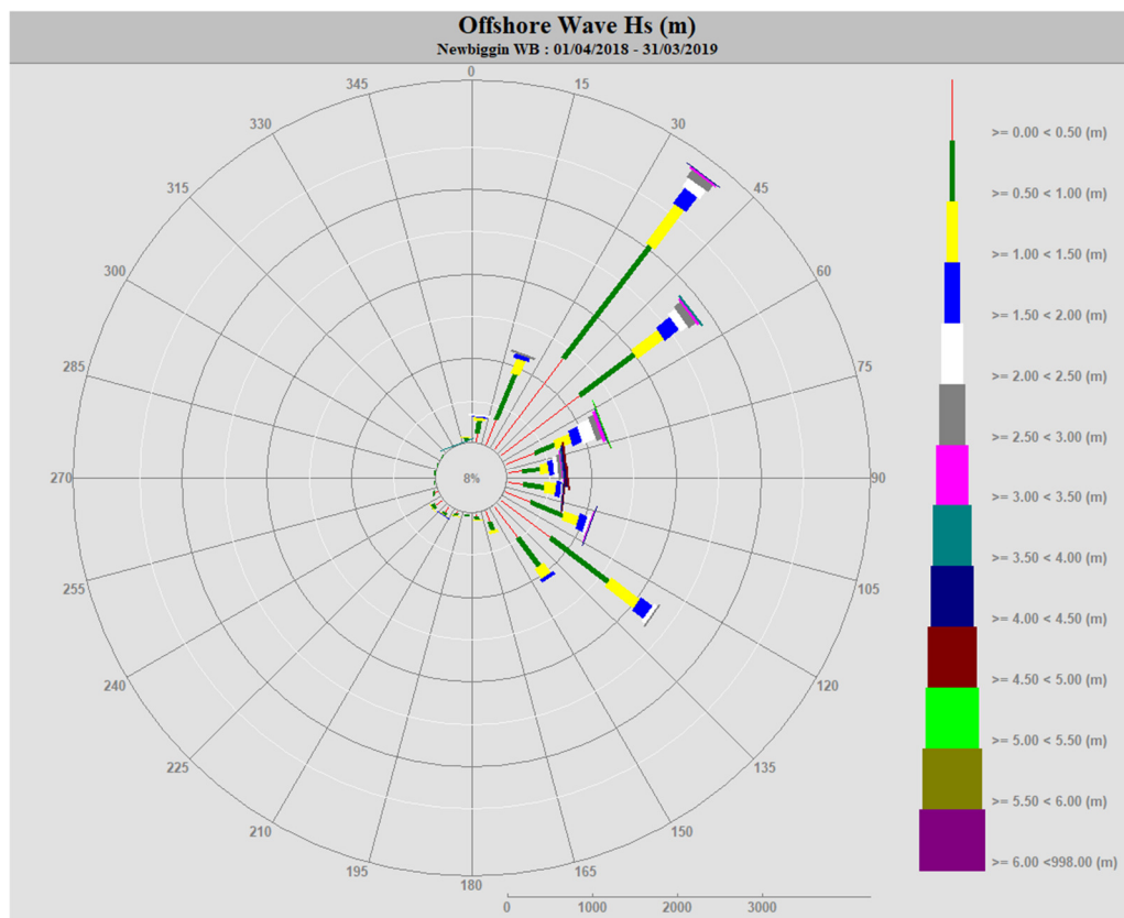
Figure 2.2 (continued) Wave roses for Newbiggin WB original deployment in 2010/11 and new data for 2013/14, 2014/15, 2015/16, 2016/17, 2017/18 and 2018/19.
