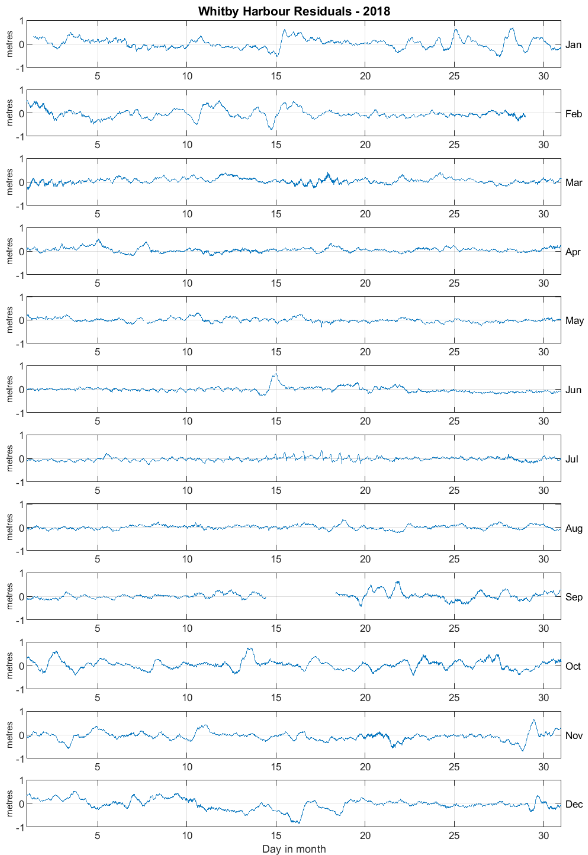
Figure 1: Whitby Harbour residuals for 2018
