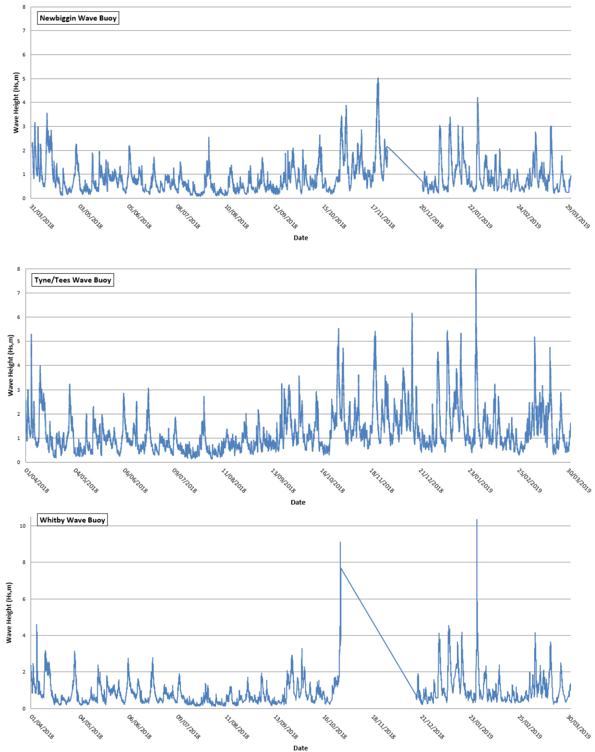
Figure 2.5 Comparison of recorded wave heights at Tyne Tees to the Cell 1 programme buoys from April 2018 to March 2019
