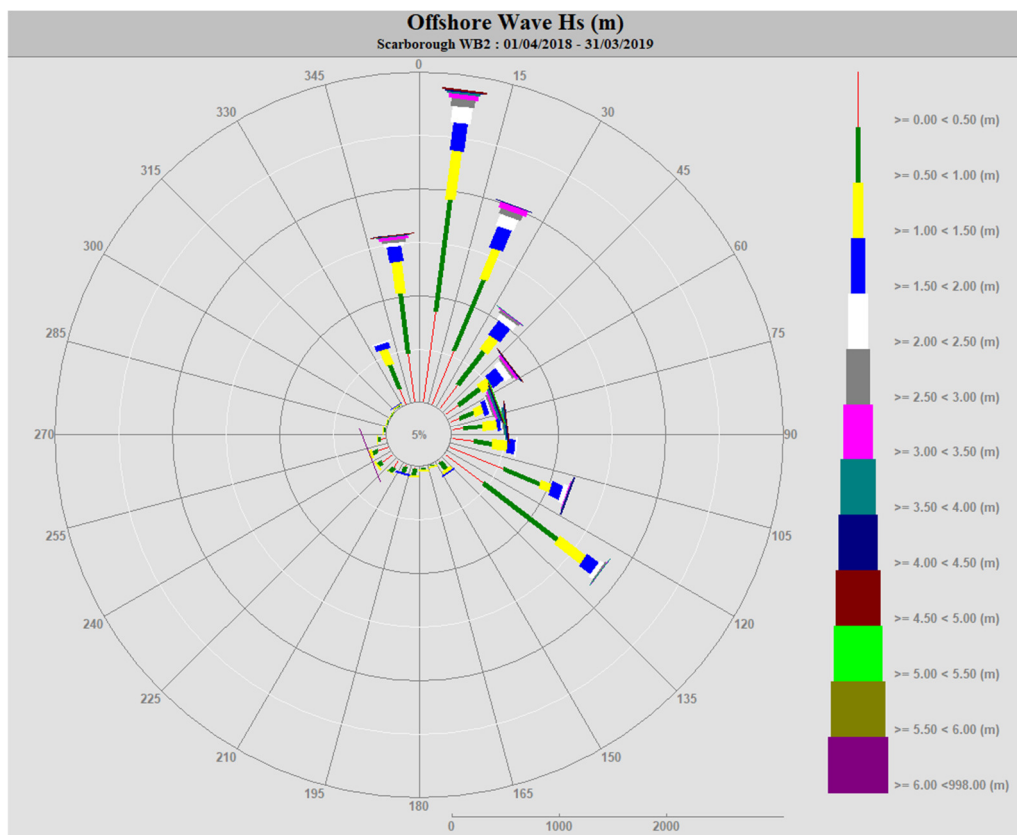
Figure 2.16 Wave Rose at Scarborough WB2 site
